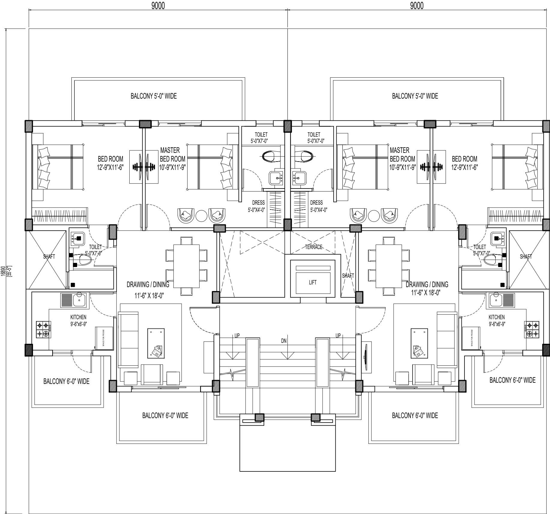
TYPICAL FLOOR PLAN (FIRST AND SECOND & THIRD)
