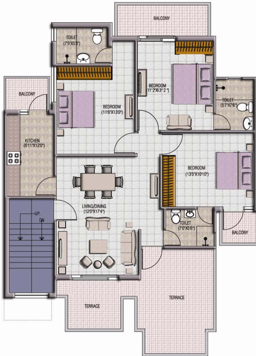
( TYPE :-A ) 300 YARDS SECOND FLOOR PLAN
